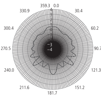
Typical ripple with dipole, average normalized (1880 MHz)
