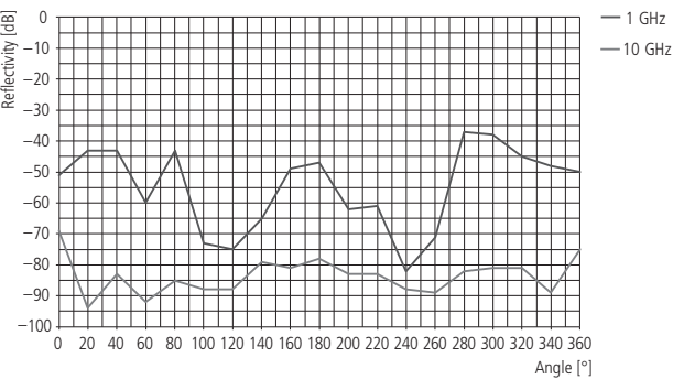
Typical QZ reflectivity 7 m distance, 2 m QZ size
